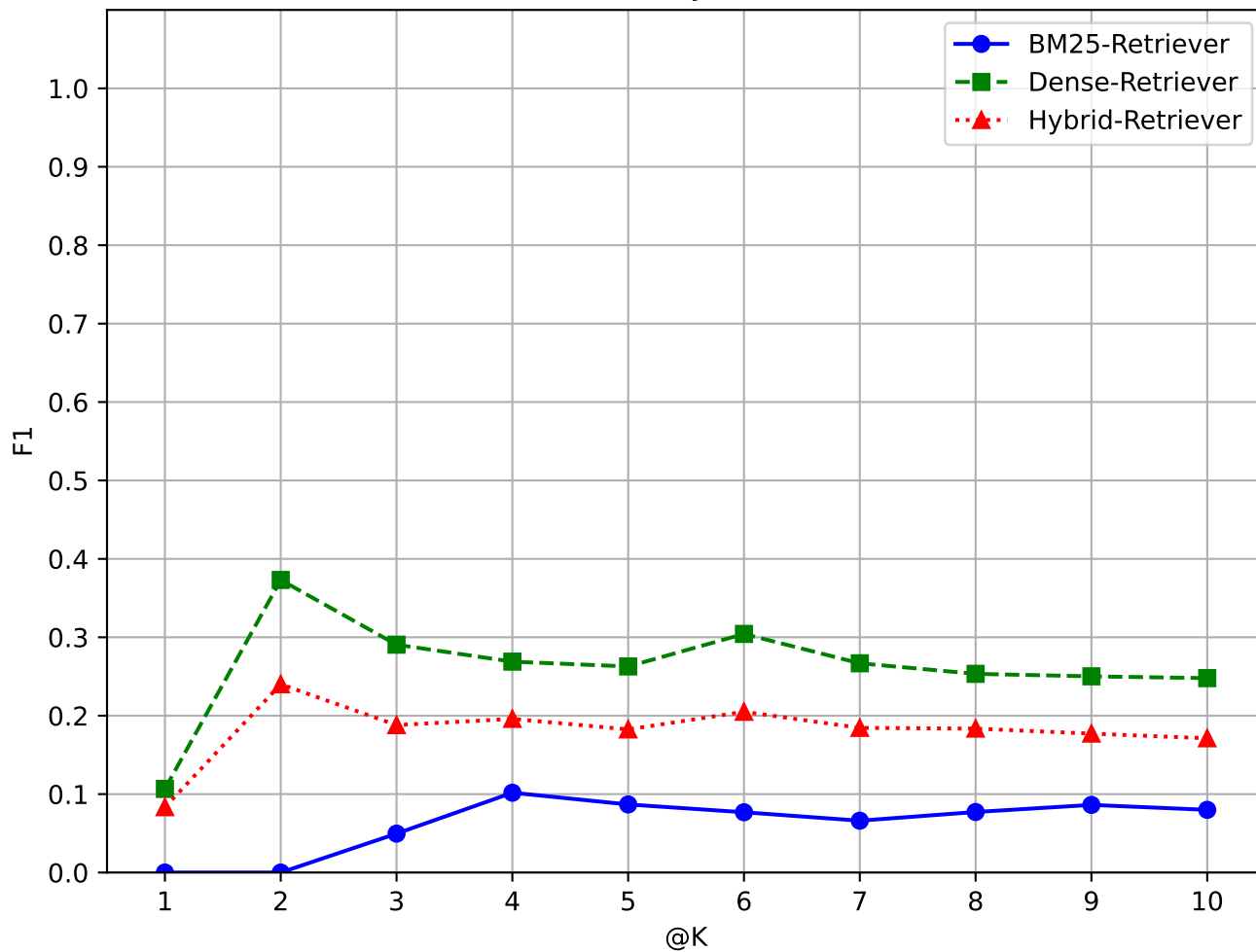
Query 37
